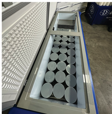
Accommodates 27 6x12" cylinders
