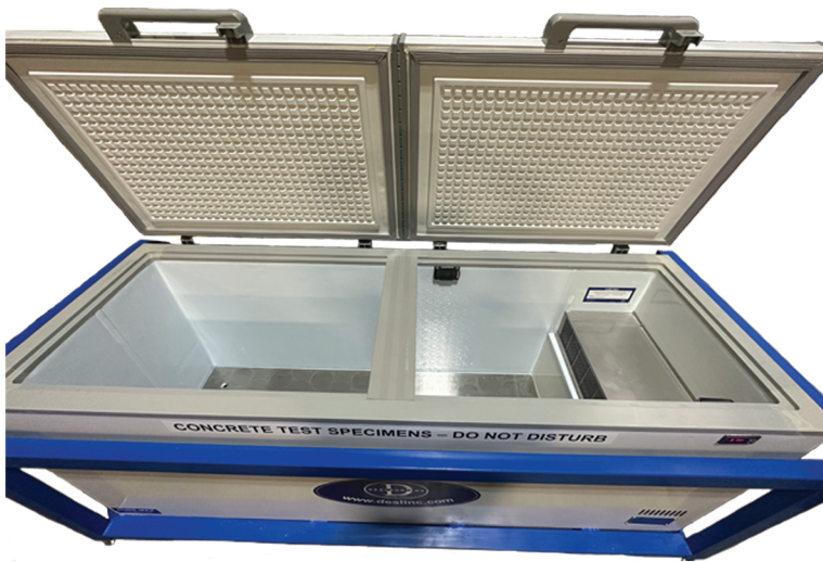
Accommodates 27 6x12" cylinders
